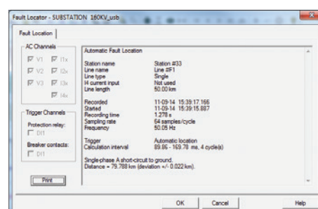
DISTANCE TO FAULT CALCULATION (PAS)
